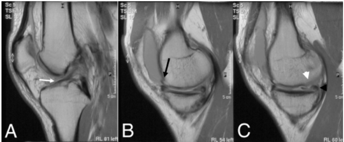
Figure 2: This sagittal T1 weighted MRI scan shows degenerative changes present in the medial compartment of the knee in a male subject with 12-year history of chronic ACL-deficiency. In the left image (A) can be seen a chronic ACL tear with attrition of remaining strands (white arrow), in the centre (B) and right images (C), medial compartment degenerative changes including osteophytes (black arrow), chronic tear of the posterior horn of the medial meniscus (black arrowhead), and damage to the articular surface of the femoral condyle (white arrowhead). There is also an effusion medial to the patella.
