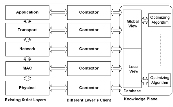
Fig. 1: Proposed Cross-Layer Architecture [1]
