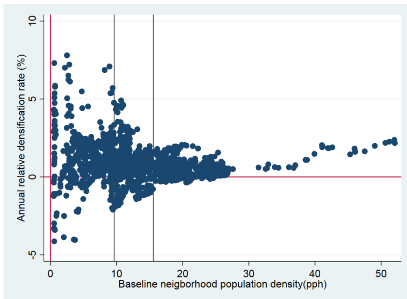
Figure S2. Scatterplots showing the relationships of annual relative population densification (top) and annual absolute population densification (bottom) with baseline population density.
